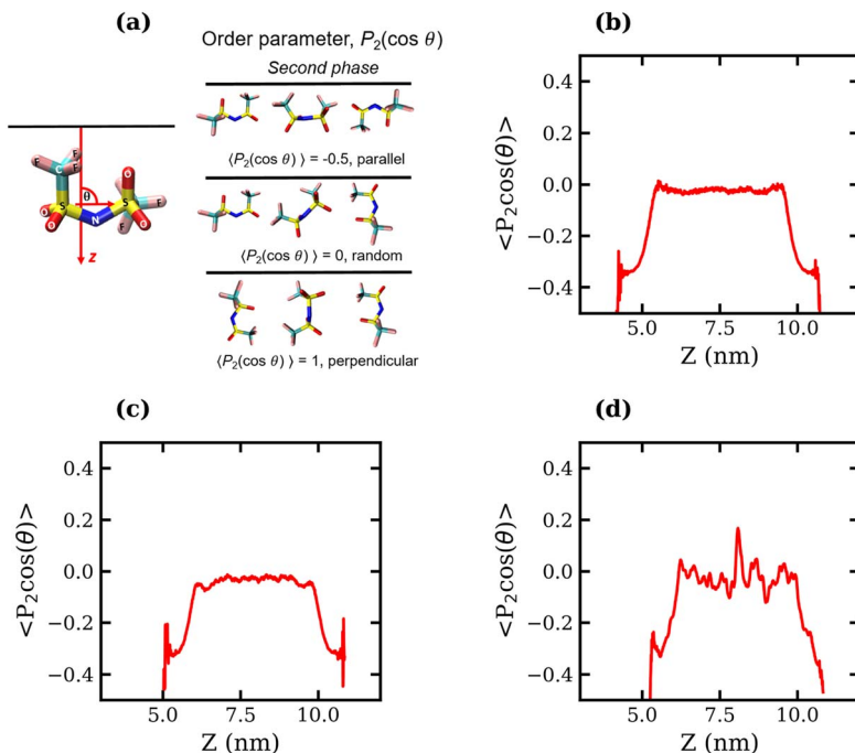
Fig. 5 Average order parameter, \langle P_2(\cos \theta) \rangle , of \text{TFSI}^- anions measured as the second Legendre polynomial of \theta , the angle between the S–S vector and interface normal (a), plotted against the Z coordinate for the (b) 1 molal, (c) 10 molal and (d) 20 molal liquid–vapour systems.
