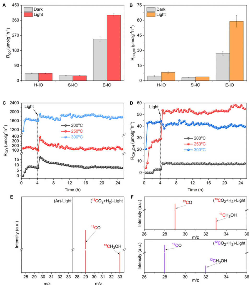
Fig. 3 \text{CO}_2 hydrogenation performance (A) \text{CO} production rate at 250 °C with and without solar irradiation. (B) \text{CH}_3\text{OH} production rate at 250 °C with and without solar irradiation. (C) Long-term (20 h) \text{CO} production over E-IO at different reaction temperatures with solar irradiation. (D) Long-term (20 h) \text{CH}_3\text{OH} production over E-IO at different reaction temperatures with solar irradiation. (E) GC-MS data from Ar and ^{13}\text{CO}_2/\text{H}_2 atmosphere under irradiation condition at 250 °C. (F) ^{13}\text{CH}_3\text{OH} and ^{13}\text{CO} obtained from ^{13}\text{CO}_2 hydrogenation, and ^{12}\text{CH}_3\text{OH} and ^{12}\text{CO} as a reference.
