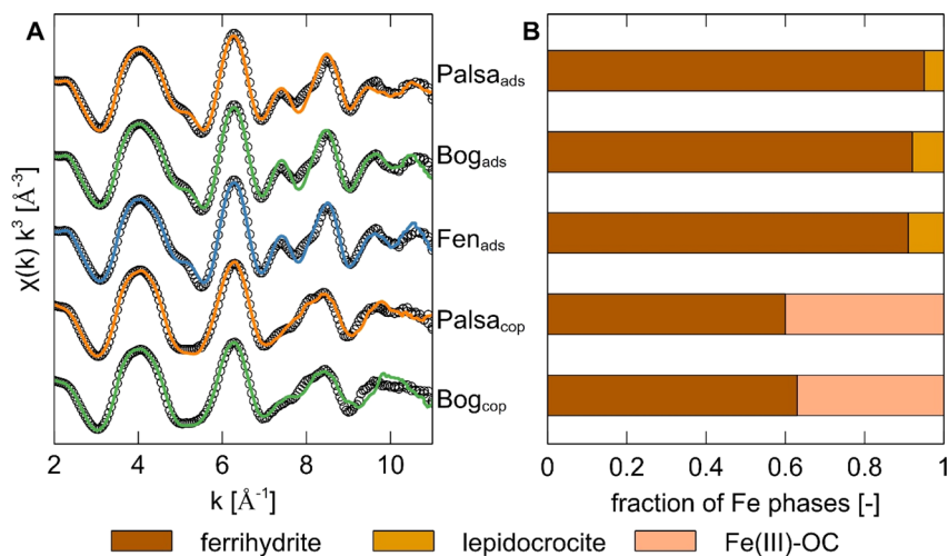
Fig. 2 (A) Iron K-edge k^3 -weighted EXAFS spectra and linear combination fits (2 to 11 \text{Å}^{-1} ) of ferrihydrite with adsorbed WEOM (ads) from palsa, bog and fen, and Fe-OC coprecipitates (cop) synthesized with WEOM from palsa and bog. Experimental data is displayed as coloured lines and linear combination fits as black circles (see fit parameters in Table S6†). (B) Bar plot showing relative abundances of different Fe phases in the post-adsorption and post-coprecipitation mineral phases. The same labelling as for graph (A) applies here. Fe(III)-OC was fit using Fe(III)-citrate as a reference.
