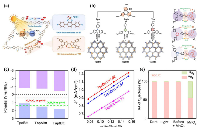
Fig. 5 (a) The mechanism behind photosynthesis of H 2 O 2 by TTF-BT-COF. 80 (b) Synthesis of TpaBtt, TapbBtt and TaptBtt and directionality of electron transfer between functional motifs and imine linkage in TpaBtt, TapbBtt, and TaptBtt. 82 (c) Energy band values of TpaBtt, TapbBtt, and TaptBtt. 82 (d) Koutecky–Levich plots of TpaBtt, TapbBtt and TaptBtt obtained by RDE measurements. 82 (e) •O 2 - yields of TpaBtt, TapbBtt and TaptBtt detected by NBT method under light conditions. 82
