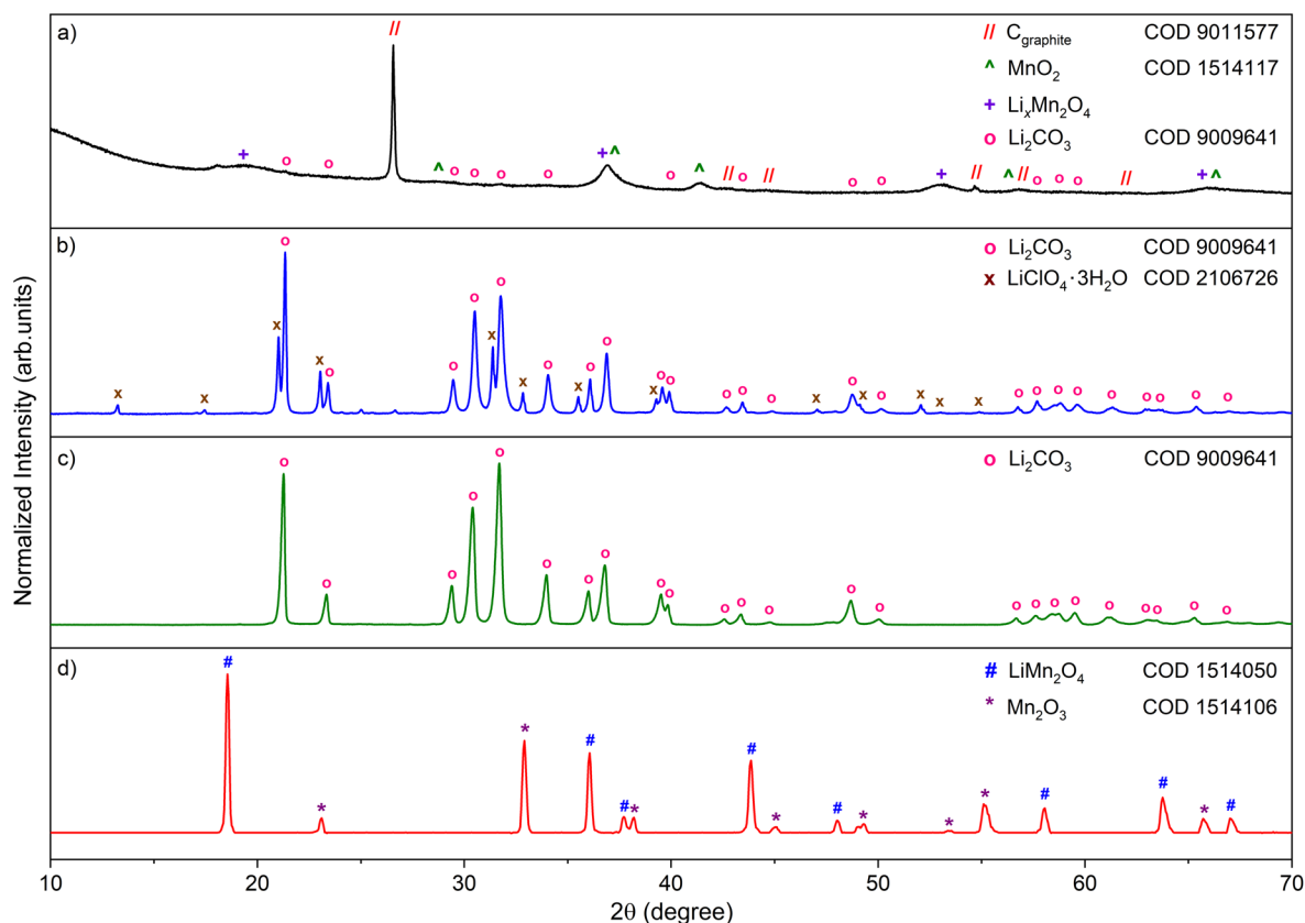
Fig. 11 PXRD patterns of the crude cathode material (a); Li 2 CO 3 /LiClO 4 ·3H 2 O mixture extracted with H 2 O and MeOH treatment (b); Li 2 CO 3 after purification with MeOH (c); and oxide materials received by means of calcination of cathode residues at 900 °C (d).
