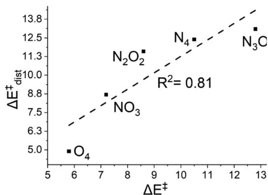
Fig. 6 A plot of activation energy ( \Delta E^\ddagger , in kcal mol -1 ) versus the distortion energies ( \Delta E^\ddagger_{\text{dist}} , in kcal mol -1 ) of the oxidants at the S = 2 state.
