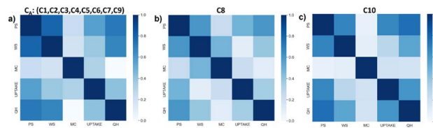
Fig. 11 Heatmap representation of the correlation coefficients of each feature corresponding to the three clusters (a) C A , (b) C8 and (c) C10 obtained from the EDDA and LDA hybrid methodology. Color codes for the correlation values.
