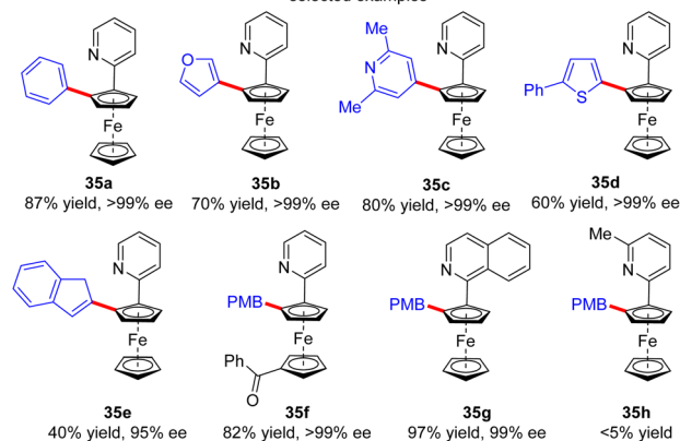
Scheme 10 Rh(I)-Catalyzed enantioselective \text{C}(\text{sp}^2)\text{-H} functionalization of ferrocenes (PMB = p -methoxybenzyl).
