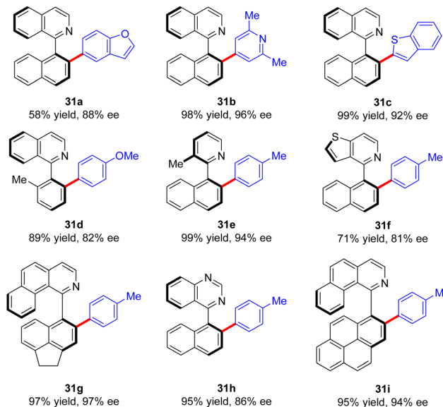
Scheme 9 Rh(I)-Catalyzed atroposelective \text{C}(\text{sp}^2)\text{-H} arylation of heteroaryls with aryl and heteroaryl bromides.
