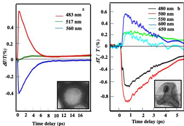
Fig. 12 Dynamics of the \Delta T/T at selected probe wavelengths, at short time scales of energy flow in the (a) Au and (b) \text{Au}(\text{Fe}_3\text{O}_4)_{13} superstructures. 27
