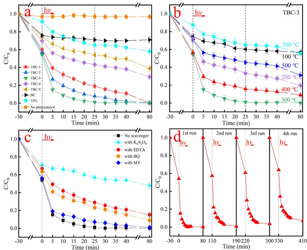
Fig. 9 Absorption-photocatalytic reduction of Cr(VI) with BC, TiO_2 and TBC samples (a), with TBC-3 calcined at different temperatures (b) and over TBC-3 composite in the presence of K_2S_2O_8 , EDTA, BQ and MT scavengers (c). Recycling experiments using TBC-3 composite for the absorption-photocatalytic reduction of Cr(VI) (d).
