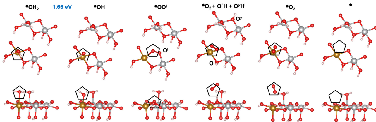
Fig. 4 Atomic structures of the intermediates involved in the OER mechanism on the Fe-doped hydrated site ( \bullet ) with the lowest overpotential on \beta -NiOOH(10 \bar{1} 0), relaxed using DFT-HSE06 ( \alpha = 15\% ). The intermediate labels are abbreviated from the labels provided in Table 3. The ONIOM Gibbs free energy change corresponding to the PDS is shown in blue. Top panels: Top-down view. Bottom panels: Side view. The empty pentagons mark the location of oxygen-containing species at the active site. O^l and O^l' denote lattice oxygen atoms in the same layer, whereas O^y denotes a lattice O in the adjacent layer of \beta -NiOOH(10 \bar{1} 0). Both O^l' and O^y participate in the proton transfer events. We show only the top layer for clarity. Brown sphere: Fe, grey: Ni, red: O, and pink: H.
