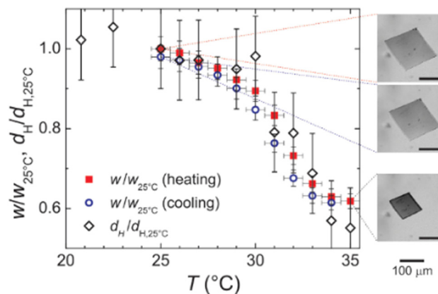
Fig. 5 Evolution of sample size with temperature of square-cut hydrogel films in water during heating (solid red squares) and cooling (open blue circles). The width w is renormed to the one at 25 ^\circ\text{C} . The normalized hydrodynamic diameter d_H/d_{H,25^\circ\text{C}} of the constituent particles is shown (open diamonds) in the same diagram ( d_H = 1.53 \mu\text{m} at 25 ^\circ\text{C} ). Pictures on the right show micrographs of the film at 25 ^\circ\text{C} (before and after heating cycle) and 35 ^\circ\text{C} , respectively. Reproduced with permission from Still et al. (2015), Temperature-Sensitive Hydrogel-Particle Films from Evaporating Drops, Adv. Mater. Interfaces , 2 (16). ©2015 WILEY-VCH Verlag GmbH & Co. KGaA, Weinheim.
