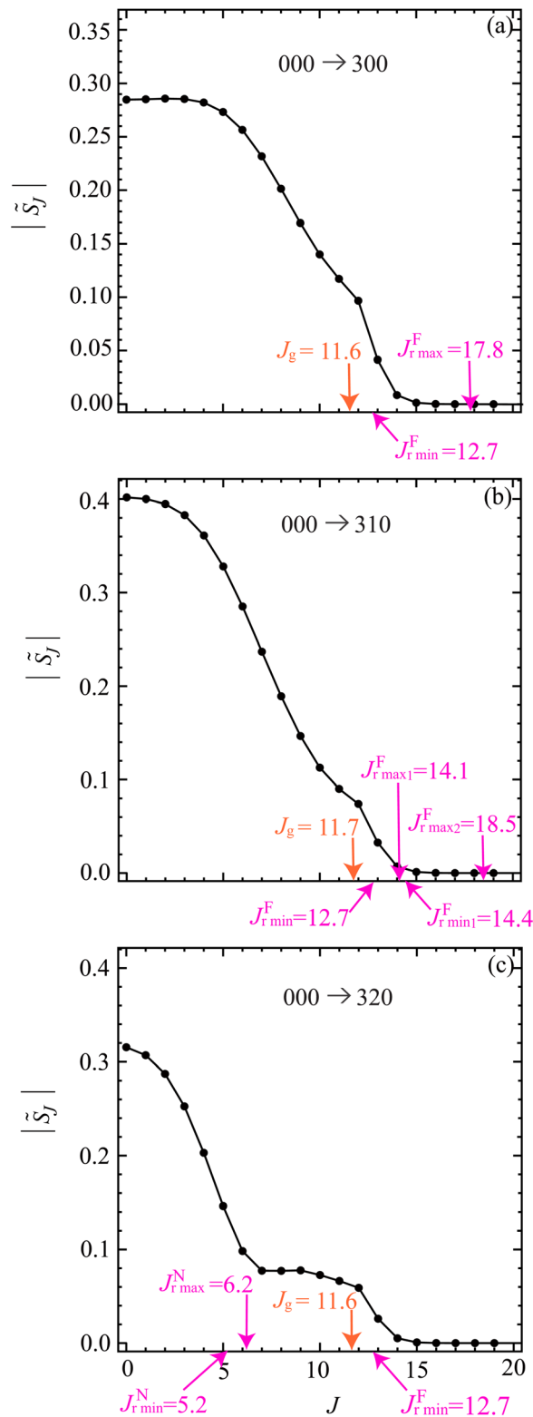
Fig. 1 Plots of |\tilde{S}_J| versus J at E_{\text{trans}} = 62.09 meV. The black solid circles are the numerical S matrix data, \{\tilde{S}_J\} , at integer values of J , which have been joined by straight lines. The orange arrow indicates the value of the glory angular momentum variable, J_g . The pink arrows indicate the values of the nearside (N) and farside (F) rainbow angular momentum variable. The notation and values of J_g , and the rainbow angular momenta, are taken from Fig. 6. The transitions are: (a) 000 \rightarrow 300 , (b) 000 \rightarrow 310 , (c) 000 \rightarrow 320 .
