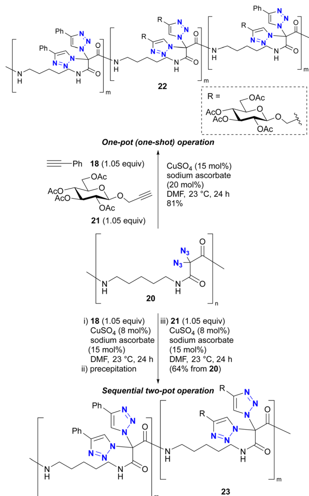
Scheme 4 CuAAC functionalization of the geminal diazide polymers and click site control.
