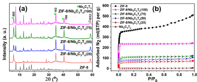
Fig. 2 (a) XRD pattern of various ZIF-8/ \text{Nb}_4\text{C}_3\text{T}_x composites. (b) \text{N}_2 adsorption isotherms of ZIF-8, \text{Nb}_4\text{C}_3\text{T}_x and their composites (the closed symbols represent adsorption, while the open symbols represent desorption).
