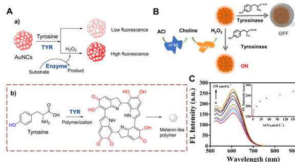
Fig. 14 (A) The response mechanism of AuNCs (a) and the generation of melanin-like polymer (b). (B) The illustration of AuNCs for ACI. (C) The fluorescence intensity spectra of AuNCs with different concentrations of ACI ( 0\text{--}150 \mu\text{mol L}^{-1} ) (reprinted with permission from ref. 51 Copyright © 2019, Elsevier).
