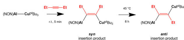
Scheme 8 Experimental insertion of internal 3-hexyne in the Cu–Al bond of the [\text{tBu}_3\text{PCuAl}(\text{NON})] complex. 68
