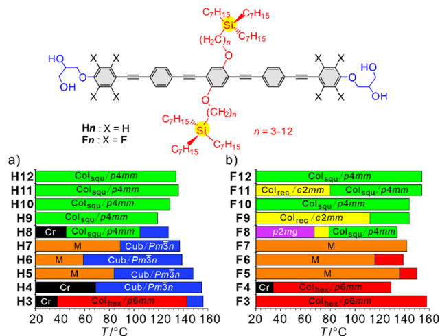
Fig. 2 Molecular structure and LC phases of (a) H n and (b) F n as observed on cooling with 10 K min -1 ; abbreviations: Cr = crystalline solid; Col hex /p6mm and Col sq /p4mm = triangular and square LC honeycombs, respectively; Col rec /c2mm and p2mg = tilings by rhombic and non-regular triangular honeycombs, respectively; Cub/Pm3n = cubic network phase with Pm3n space group; M = unknown LC phases; isotropic liquid is at the right side of the columns; for numerical data, transitions on heating and enthalpies, see Table S1a, b, for DSCs Fig. S1 and S2, for textures Fig. S3–S6, for SAXS/WAXS data Fig. S7–S10, Tables S2–S29 (ESI†).
