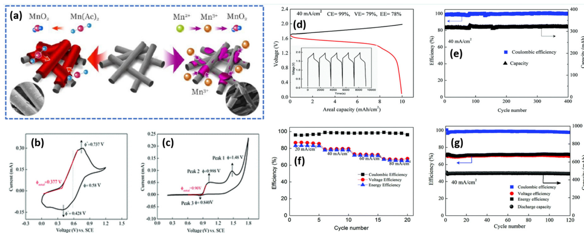
Fig. 12 (a) Schematic representation of the electrochemical performance of \text{MnO}_2 and \text{MnSO}_4 electrolyte, cyclic voltammetry profile of the glassy carbon electrode recorded at a scan rate of 10 \text{ mV s}^{-1} in (b) 0.05 \text{ M Mn(Ac)}_2 in 1 \text{ M KCl} and (c) 0.05 \text{ M MnSO}_4 in 0.5 \text{ M K}_2\text{SO}_4 , (d) GCD profile of Zn/Mn RFB recorded at 40 \text{ mA cm}^{-2} , (e) capacity retention and the coulombic efficiency plot with 7 \text{ mA h cm}^{-2} , (f) the rate capability of Zn/Mn RFB observed at different current density, and (g) cyclability of Zn/Mn RFB with 10 \text{ mA h cm}^{-2} at 40 \text{ mA cm}^{-2} (reproduced from ref. 34 with permission from The Royal Society of Chemistry).
