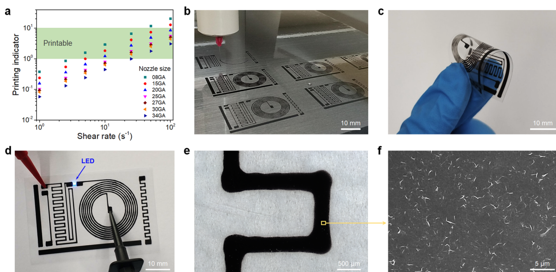
Fig. 4 (a) Printing indicator of the graphene inks ( 10\ mg\ mL^{-1} ) at different shear rates. (b) Printing of multiple flexible conductive circuit patterns. (c) Bending of the printed flexible conductive circuit without failure. (d) Lighting up of an LED chip on the printed flexible conductive circuit. (e) The optical microscopy image of a printed line. (f) The corresponding SEM image of the printed pattern.
