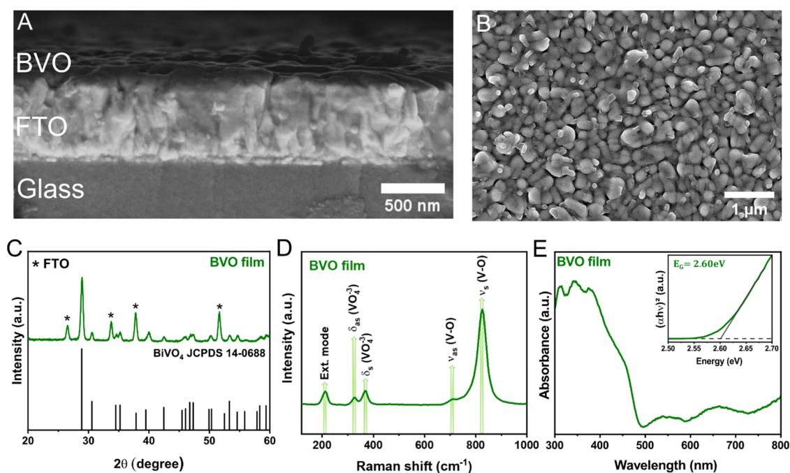
Fig. 1 Characterization of bare BVO film deposited for 8 minutes and calcined at 400° for 1 hour: (A) cross-section SEM images, (B) Top view SEM images, (C) XRD patterns, (D) Raman spectrum and (E) UV-vis absorption spectrum, inset: Tauc Plot analysis.
