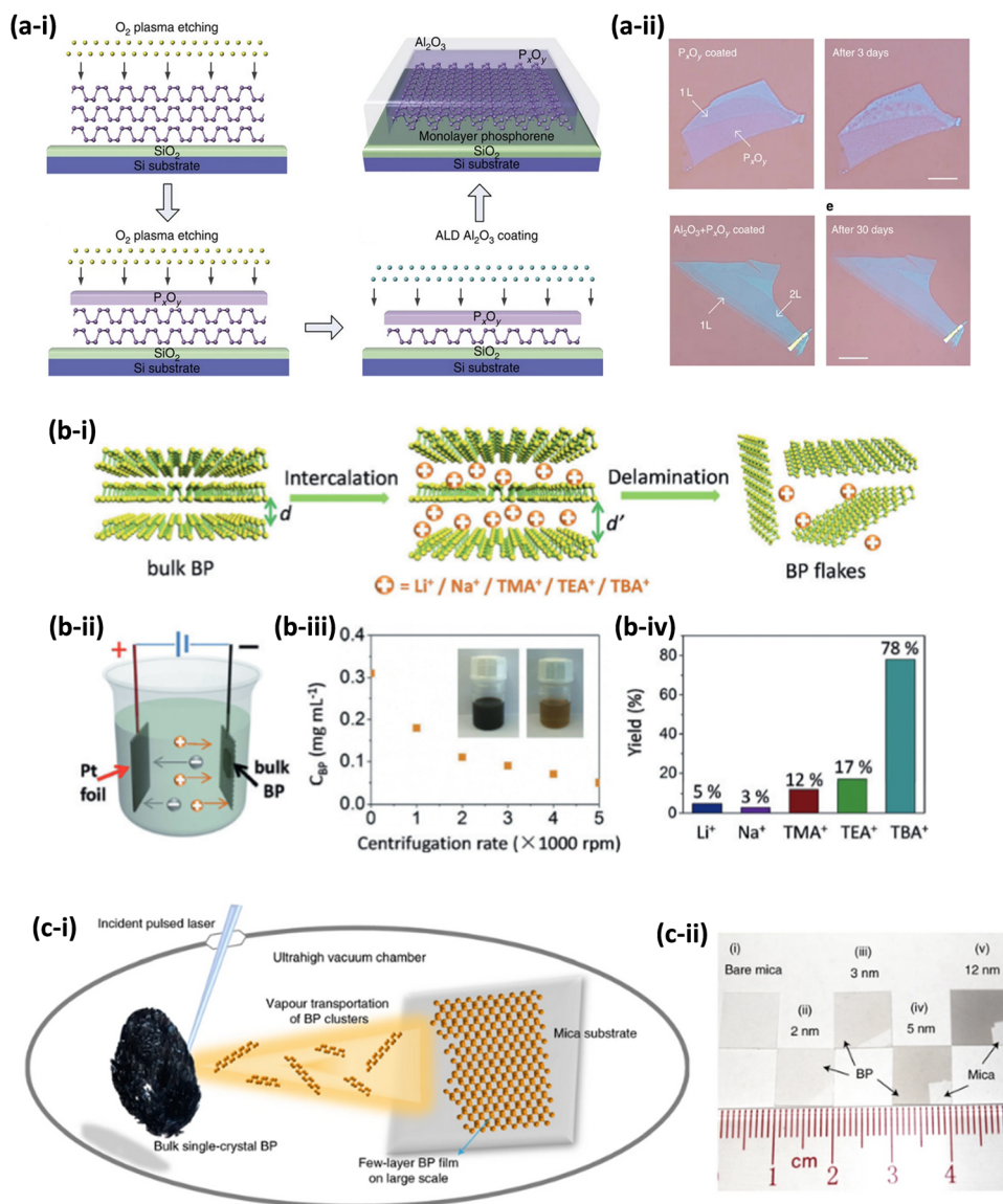
Fig. 8 (a) Mechanically exfoliated black phosphorus (BP) on a SiO_2/Si substrate treated with O_2 plasma etching: (a-i) schematic illustration of the preparation process, and (a-ii) OM images of single-layer BP covered by P_2O_5 or P_2O_5/Al_2O_3 capping layer before and after several days. 109 Reproduced with permission from ref. 109. Copyright 2016, Springer Nature. (b): Electrochemically exfoliated BP: (b-i) Schematic delamination procedure, (b-ii) Experimental setup, (b-iii) Concentration of BP as a function of centrifugation rate, and (b-iv) Delamination yield as a function of intercalating cations. 125 Reproduced with permission from ref. 125. Copyright 2016, John Wiley-VCH.
