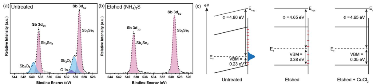
Fig. 3 Synchrotron-based XPS core level spectra of Sb 3d for (a) untreated Sb 2 Se 3 and (b) Sb 2 Se 3 etched with (NH 4 ) 2 S. (c) Band alignment changes due to the Sb 2 O 3 layer (represented by the blue Gaussian) and surface states (represented by red dashes), measured by KP-FM and XPS valence band maxima (VBM). Band bending is represented as a sloping line due to the low doping (the space charge region is larger than the film thickness).
