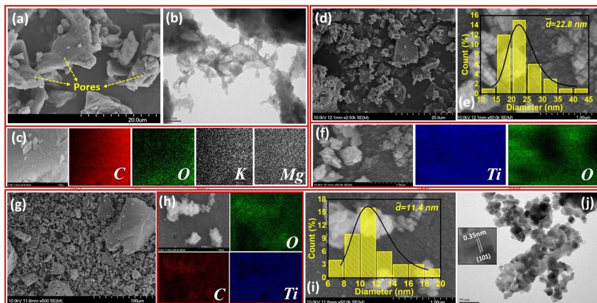
Fig. 1 (a) SEM image, (b) TEM image, and (c) EDS maps of spent-coffee ground biochar (CGB); (d) SEM image, (e) particle size distribution and (f) EDS maps of \text{TiO}_2 ; and (g) SEM image, (h) EDS mapping, (i) particle size distribution and (j) TEM image of CGBT nanocomposites.
