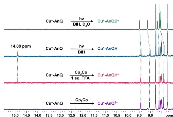
Fig. 7 Comparison of the ^1\text{H} NMR spectra of \text{Cu}^+-\text{AnQ}^{2-} (purple line), \text{Cu}^+-\text{AnQH}^\bullet generated by \text{Cp}_2\text{Co} and 1 eq. trifluoroacetic acid (red line), \text{Cu}^+-\text{AnQH}^\bullet generated by 30 minutes illumination with BIH (teal line), \text{Cu}^+-\text{AnQD}^{\bullet-} generated by BIH with 30 min illumination and then added with one drop of \text{D}_2\text{O} (green line). Illumination with 455 nm light; concentrations of the complex and BIH were kept at 0.2 mM and 0.1 M, respectively, in \text{CD}_3\text{CN} .
