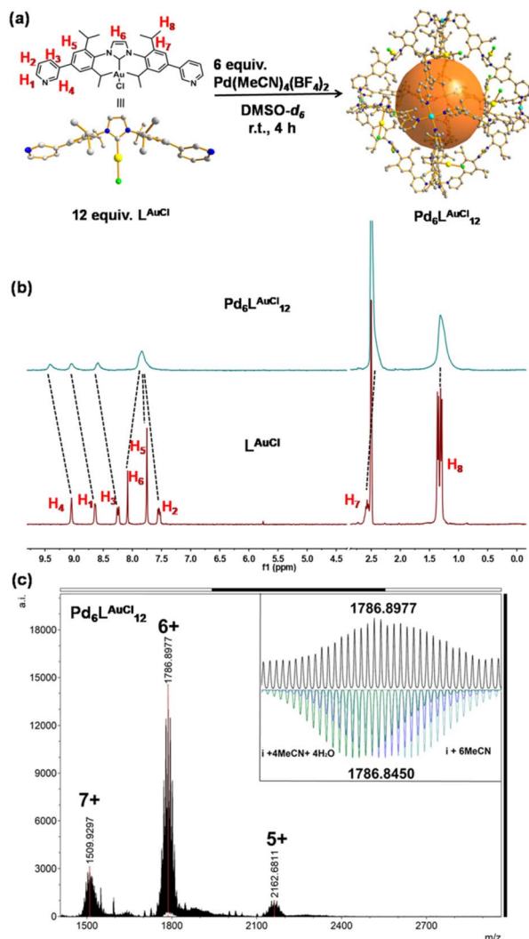
Fig. 3 Synthesis and characterization of \text{Pd}_6\text{L}_{12}\text{AuCl}_{12} . (a) Synthesis of the self-assembly of \text{Pd}_6\text{L}_{12}\text{AuCl}_{12} . The structures of \text{L}^{\text{AuCl}} and \text{Pd}_6\text{L}_{12}\text{AuCl}_{12} are obtained by SCXRD. (b) ^1\text{H} NMR of \text{L}^{\text{AuCl}} and the \text{Pd}_6\text{L}_{12}\text{AuCl}_{12} in \text{DMSO-d}_6 (at 298 K). Color coding: C: gray; N: dark blue; Au: yellow; Pd: light blue; Cl: bright green; B: dark green; F: violet; O: red; H: white. (c) HR-ESI-MS of \text{Pd}_6\text{L}_{12}\text{AuCl}_{12} and simulated isotopic distribution of charged species (+6) containing solvent molecules.
