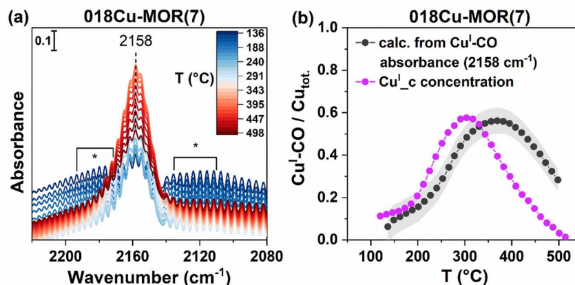
Fig. 9 (a) FT-IR spectra obtained during CO-TPR. Spectra are background subtracted. (b) A comparison of the fraction of \text{Cu}^{\text{I}} -CO species found with XAS throughout the TPR protocol ( \text{Cu}^{\text{I}}_{\text{c}} ), and the corresponding \text{Cu}^{\text{I}} -monocarbonyl fraction calculated from Lambert–Beer law by integrating the band at 2158\text{ cm}^{-1} . The error bars (grey band) are given as the standard deviation determined from three different baseline positions on the rotational–vibrational features when obtaining the integrated area.
