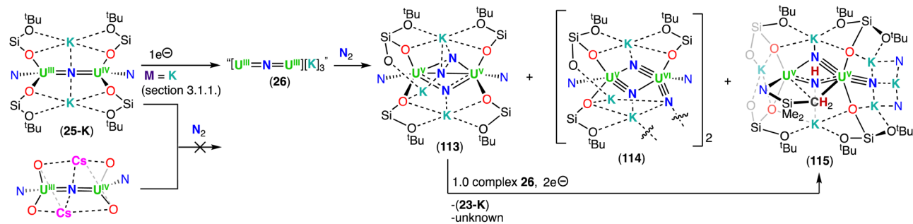
Scheme 23 Reactivity of U(III)-bridged nitrides supported by amide (-N(SiMe 3 ) 2 ) and siloxide (-OSi(O t Bu) 3 ) ligands. Most of the -O t Bu moieties of the ligand have been omitted for clarity.
