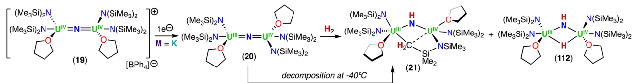
Scheme 22 Reactivity of U(III)-bridged nitrides supported by amide (-N(SiMe 3 ) 2 ) ligands.
