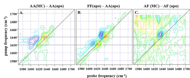
Fig. 3 (A) shows the difference spectrum obtained by subtraction of IL-17AA apo-2D-IR data from a 1:2 macrocycle (MC) bound sample at waiting time ( T_w ) of 250 fs and at parallel polarisation, whilst (B) shows the subsequent difference obtained from subtraction of the same IL-17AA apo-data from that for an IL17-FF apo-sample at the same waiting time. A similar difference is shown in (C), obtained for an AF macrocycle minus AF apo-subtraction, again at a T_w of 250 fs, but with a much lower signal-to-noise level that is indicative of the low binding affinity of the AF isoform. The dashed horizontal lines highlight the similarity in peak positions for both subtractions, indicating that the binding of the macrocycle to both IL-17AA and IL-17AF induces changes that are much more comparable both spectroscopically and structurally to the IL-17FF apo-form.
