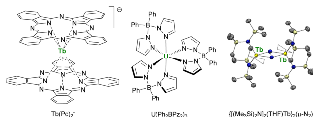
Fig. 6 Molecular structures of \text{Tb}(\text{Pc})_2^- , 70 \text{U}(\text{Ph}_2\text{BPz}_2)_3 , 176,177 and ORTEP plot of [(\text{Me}_3\text{Si})_2\text{N}]_2(\text{THF})\text{Tb}_2(\mu\text{-N}_2)^- , 180 (terbium atoms are in yellow, nitrogen atoms in blue, silicon atoms in pale yellow, carbon atoms in grey, hydrogen atoms are not represented, and coordinated thf molecules are represented in wireframe).
