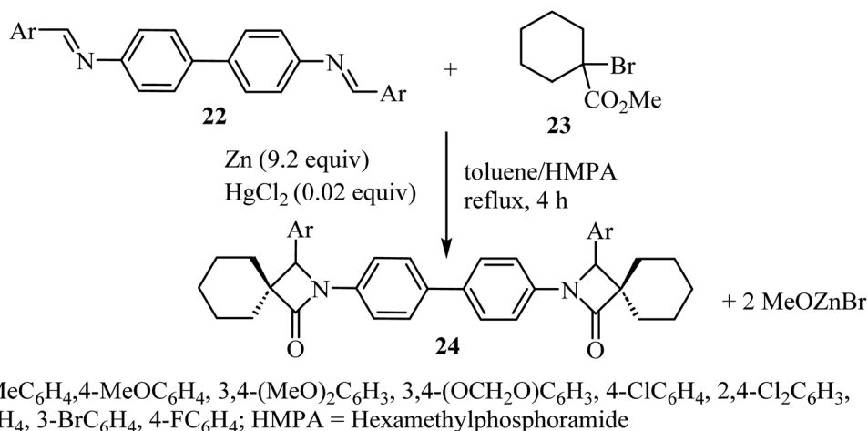
Scheme 6 Zinc mediated reaction between N,N -bis(arylmethyldene)benzidines 22 and an \alpha -bromoalkancarboxylate 23.
