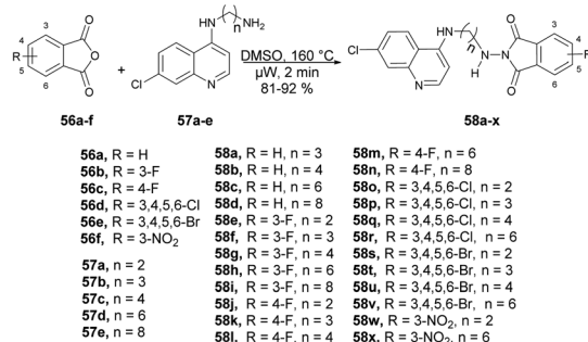
Scheme 20 Synthesis of 4-aminoquinoline-phthalimides 58a–x .
