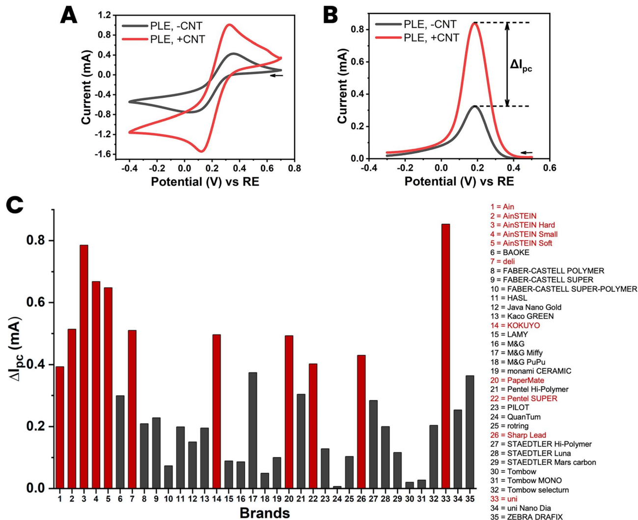
Fig. 3 Cyclic (A) and differential pulse (B) voltammograms of 100 mM ferricyanide at a HB-PL electrode (PL brand: AinSTEIN) without (black) and with (red) CNT modification. (C) A bar chart of the current increase induced by the proposed CNT modification of HB-PLEs, for all 35 PL brands tested. The supporting electrolyte for the measurements was 100 mM KCl, the scan speed for CV acquisition was 50 mV s -1 and the pulse size and time for DPV recordings were 50 mV and 200 ms, respectively. The EC cell was arranged as shown in Fig. 1(D), with a coiled Pt counter-electrode and an Ag/AgCl/3 M KCl reference.
