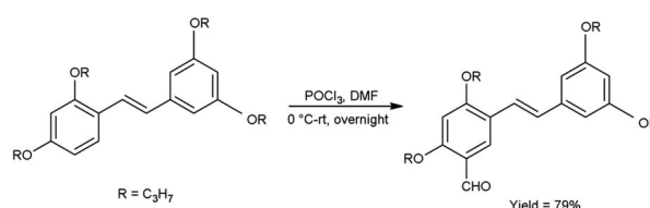
Scheme 75 Synthesis of 2'-formyl-2,3',4,5'-tetraoisopropoxystilbene.
