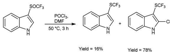
Scheme 45 Synthesis of trifluoromethylsulfonylation.
