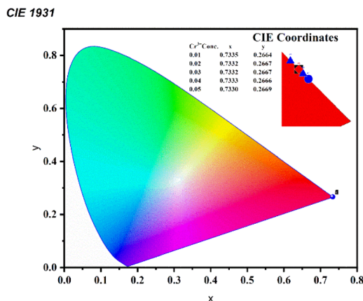
Fig. 7 CIE 1931 plot of the Cr³⁺-doped CAZ phosphor.
