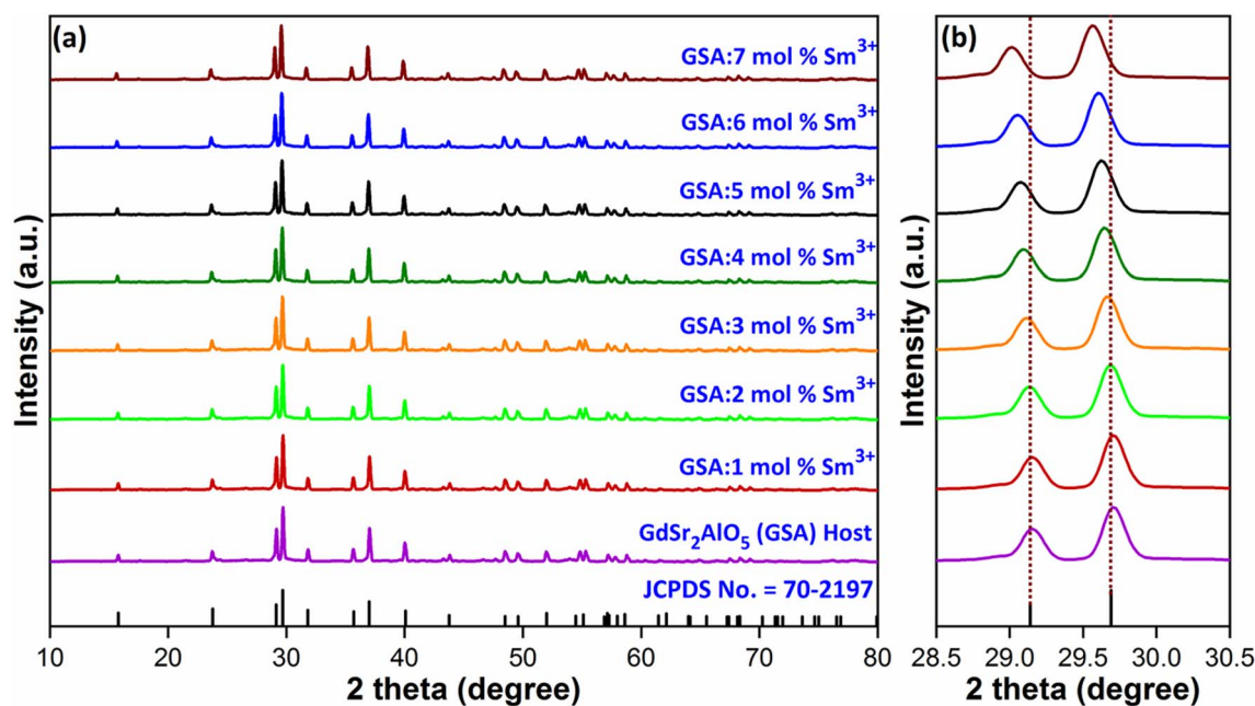
Fig. 2 (a) Diffraction profiles of \text{GdSr}_2\text{AlO}_5 and \text{Gd}_{1-x}\text{Sr}_x\text{AlO}_5:x\text{Sm}^{3+} ( x = 1-7 \text{ mol\% Sm}^{3+} ) phosphors (b) enlarged view of respective diffraction patterns.
