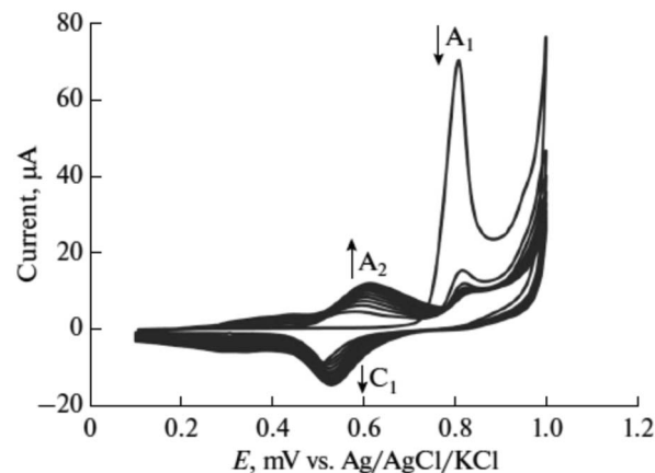
Fig. 22 Electropolymerizing process of luminol voltammogram in 0.5 \text{ M} sulfuric acid under 50 \text{ mV s}^{-1} and for 10 cycles. This figure has been adapted/reproduced from ref. 59 with permission from Springer Nature via CCC marketplace, copyright (2023).
