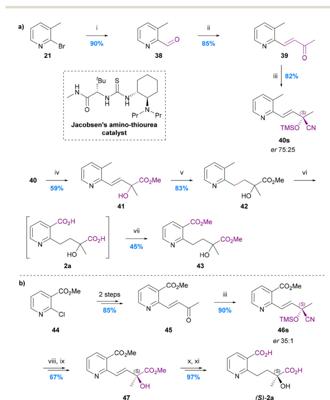
Chart 9 The synthesis of hydroxy wilfordic acid 2a . (a) Seo et al. 2009, 64 (i) n BuLi, DMF, THF, (ii) MeCOCH 2 P(O)(OMe) 2 , NaH, THF, (iii) Jacobsen's amino-thiourea catalyst, TMSCN, CF 3 CH 2 OH, CH 2 Cl 2 , –78 °C, (iv) 6 M HCl, MeOH, reflux, (v) H 2 , Pd/C, MeOH, (vi) KMnO 4 , H 2 O, reflux, (vii) HCl, MeOH; (b) Seo et al. 2019, 20 (viii) c. HCl, MeOH, 60 °C, (ix) TMSCHN 2 , MeOH, (x) H 2 , Pd/C, MeOH, (xi), LiOH·H 2 O, MeOH/H 2 O.
