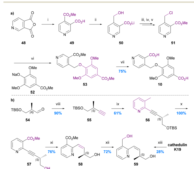
Chart 10 The synthesis of cathic acid 10 and edulinol 59 . (a) Stein and Nencini 1989, 48 (i) MeOH, (ii) LiAlH 4 , THF, (iii) POCl 3 , PCl 5 , (iv) MeOH, (v) pH 7.4, (vi) MeOH, (vii) 4 N KOH, MeOH; (b) White et al. 1993, 49 (viii) (MeO) 2 POCHN 2 , t BuOK, THF, (ix) methyl 2-chloronicotinate, (Ph 3 P) 2 PdCl 2 , Cul, Et 2 NH, (x) 5% HF/MeCN, (xi) H 2 , Lindlar cat., MeOG, (xii) LiAlH 4 , THF, 0 °C, (xiii) LiAlH 4 , THF/Et 2 O, 0 to 25 °C.
