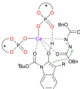
Fig. 10 Enantioselective amination of 3-aryl-2-oxindoles catalyzed by a Ca-bisphosphate. 38
