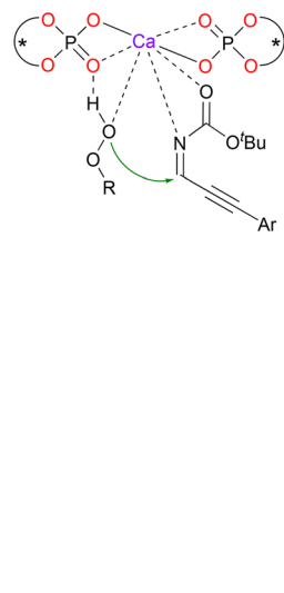
Fig. 12 Enantioselective peroxidation of C-alkynyl imines catalyzed by a Ca-bisphosphate. 40
