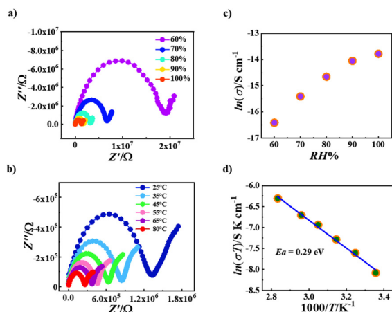
Fig. 6 Nyquist plots for R -1 at 25^\circ\text{C} under different relative humidity (RH) levels (a). Nyquist plots for R -1 at different temperatures under 100% relative humidity (RH) (b). Plots of proton conductivity vs. RH for R -1 at 25^\circ\text{C} (c). Plots of \ln(\sigma T) vs. 1000/T for R -1 under 100% relative humidity (RH) (d).
