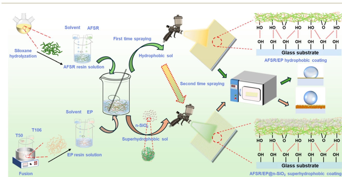
Scheme 1 The fabrication process of AFSR/EP hydrophobic coating and AFSR/EP@n-SiO 2 superhydrophobic coating.
