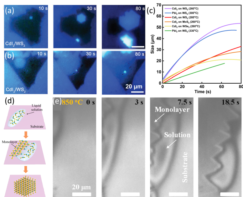
Fig. 3 Schematic illustration of in situ imaging the growth rate of M 12 (M = Cd, Pb) and MoS 2 . (a) In situ real-time images of the growth process of CdI 2 /WS 2 heterostructure at a growth temperature of 285 °C. (b) In situ real-time images of the growth process of CdI 2 /WS 2 heterostructure at a growth temperature of 260 °C. (c) Plotting of the size of M 12 (M = Cd, Pb) with time at different temperatures. Reproduced from ref. 76 with permission from Wiley, copyright 2021. (d) Illustration of the LPEE process of TMDs. (e) In situ imaging of LPEE of MoS 2 monolayers from the CsCl solution at 850 °C. Reproduced from ref. 78 with permission from American Chemical Society, copyright 2023.
