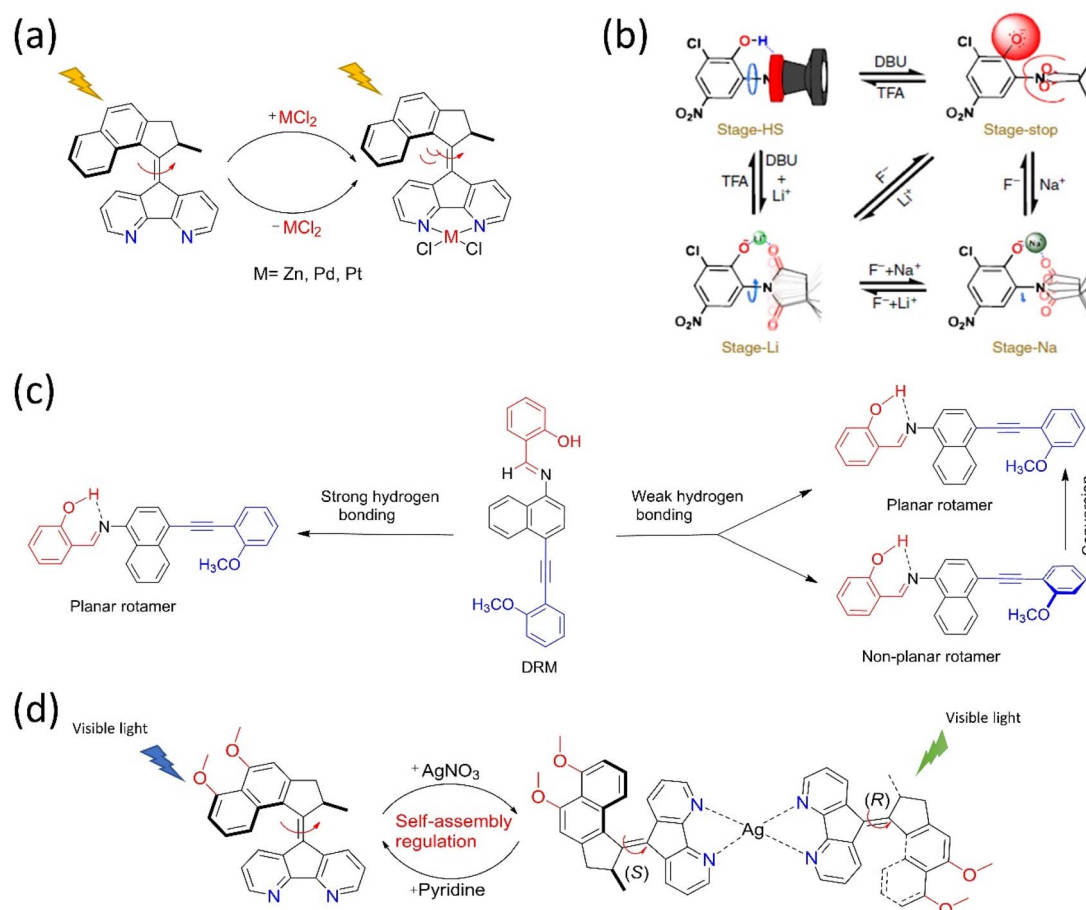
Fig. 4 Approaches for controlling the dynamic motions in molecular motors. (a) Allosteric regulation of the overcrowded alkene-based motor by incorporating Zn, Pd, and Pt metal chlorides under light. 85 (b) Schematic representation of a multistage modulated rotor, in which the four dynamic stages of the rotors are achieved with acid–base and allosteric interaction. Reproduced with permission. 87 Copyright 2018, The Authors, published by Springer Nature. (c) The rotational control of DRM by weak and strong hydrogen bonding. The “BR”, “PS”, and “AM” moieties are colored blue, black, and red, respectively. 89 (d) Coordination-directed self-assembly of a motorized nanocar. 92
