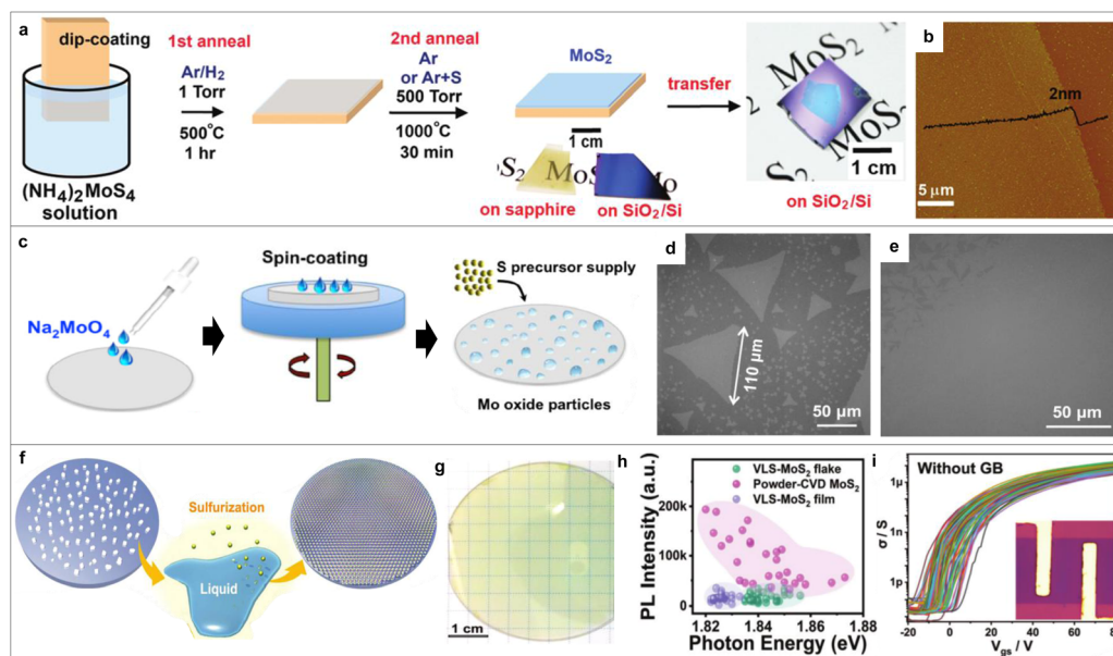
Fig. 1 (a) Illustration of the synthesis of MoS 2 layers. Inset is the optical image of MoS 2 film. 50 (b) AFM image of the triple MoS 2 . 50 (c) Illustration of the synthesis of monolayer MoS 2 . 36 (d) Optical image of MoS 2 flake. 36 (e) Optical image of continuous MoS 2 film. 36 (f) Illustration of the V-S-L growth mechanism for MoS 2 films. 52 (g) Optical image of monolayer MoS 2 film on a sapphire substrate. 52 (h) PL distribution of three types of MoS 2 samples. 52 (i) Transport curves of FETs based on MoS 2 without the growth of GB. 49 (a) and (b) Reprinted from ref. 50 Copyright 2012, the American Chemical Society. (c)–(e) Reprinted from ref. 36 Copyright 2019, Springer Nature. (f)–(i) Reprinted from ref. 52 Copyright 2019, The Royal Society of Chemistry.
