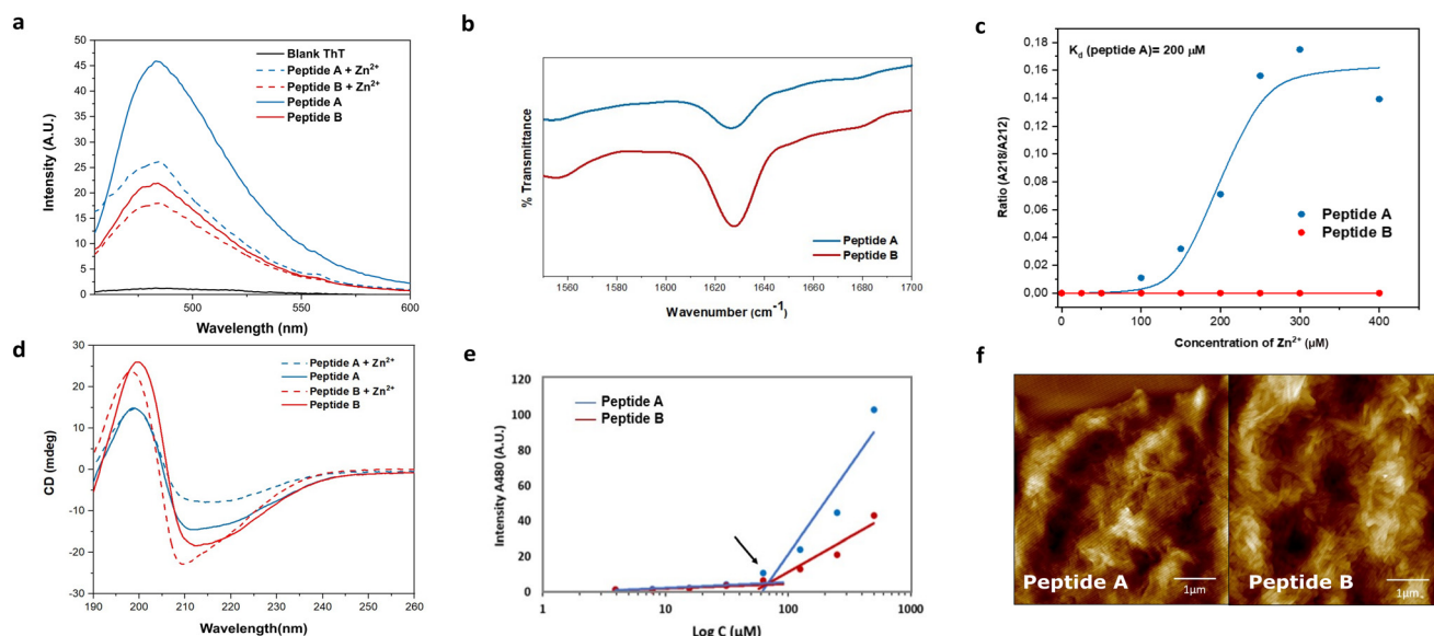
Fig. 2 Characterization of linear peptides: (a) ThT assay for peptides A (blue) and B (red) with \text{Zn}^{2+} (dashed line) and without \text{Zn}^{2+} (solid line) performed at 250\ \mu\text{M} peptide concentration. (b) ATR-FTIR spectra of peptide A and peptide B showing a peak at 1623\ \text{cm}^{-1} indicating the presence of \beta -sheets. (c) \text{Zn}^{2+} titration curve of peptide A (blue) and peptide B (red), demonstrating the differential affinity for the metal. Peptide A exhibits strong metal binding with a binding constant ( K_d ) of 200\ \mu\text{M} , while peptide B shows no affinity. (d) CD spectra of peptide A ( 25\ \mu\text{M} ) and peptide B ( 25\ \mu\text{M} ) with and without \text{Zn}^{2+} , indicating the presence of \beta -sheet assemblies in both peptides. (e) CAC in MilliQ water, plotted for different concentrations of both peptides as a function of ThT fluorescence emission at 480\ \text{nm} . (f) AFM images showing fibrillar morphologies for peptide A (left) and peptide B (right), recorded at a concentration of 250\ \mu\text{M} (scale bar: 1\ \mu\text{m} ).
