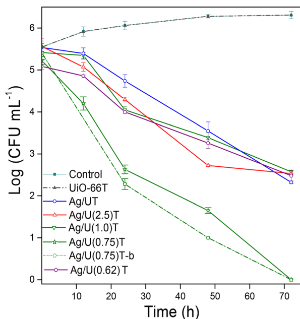
Fig. 6 Colony growth curves (CFU mL -1 ) of P. roqueforti at different incubation times, using Ag/UiO-66 solids.
