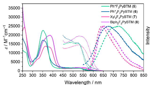
Fig. 3 Absorption (solid line) and emission (broken line, \lambda_{\text{ex}} = 450 \text{ nm} ) spectra of Ph*F 2 PyBTM (5) , Ph* 2 F 2 PyBTM (6) , Xyl 2 F 2 PyBTM (7) , and Biph 2 F 2 PyBTM (8) in dichloromethane. Enlarged portions of the absorption spectra (10 fold) are shown from \lambda = 450 to 650 \text{ nm} (dotted lines).
