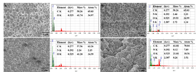
Fig. 3 Characterization of the morphology and size distribution of NPs. The scanning electron microscopy (SEM) images (scale bar: 1 \mu m) of (a) PLGA NPs, (b) ICG-loaded PLGA NPs, (c) Dox-loaded PLGA NPs and (d) Dox-ICG-loaded PLGA NPs. Representative energy dispersive X-ray (EDX) spectroscopy analysis for the elemental (C, carbon; N, nitrogen; O, oxygen; S, sulphur) compositions of the respective samples.
