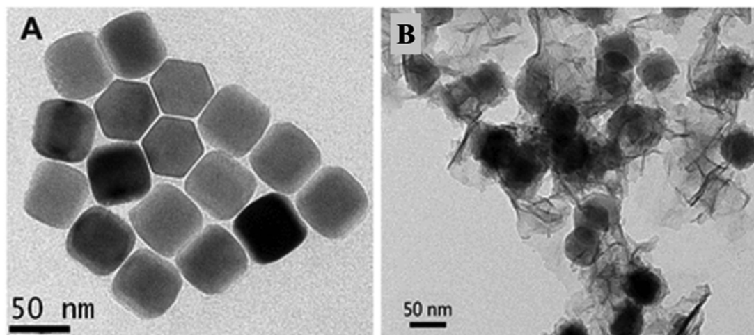
Fig. 13 TEM images (A) of OA-capped NaYF 4 :Yb,Tm@NaYF 4 core shell UCNP, and (B) of MnO 2 NS-modified NaYF 4 :Yb,Tm@NaYF 4 UCNP assemblies. 67 Copyright©2015, American Chemical Society.
