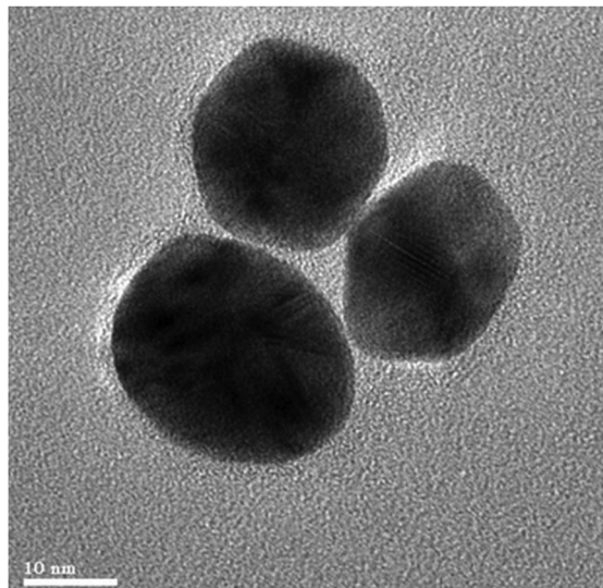
Fig. 5 HR-TEM images of guavanoic acid functionalized with Au NPs. Reproduced from ref. 53 with permission from the Royal Royal Society of Chemistry.
