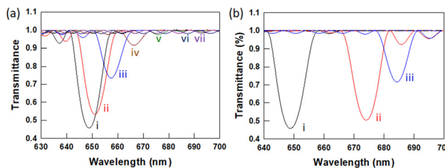
Fig. 4 Simulation of (a) H-PSLC grating transmittance at different values of the averaged director angle \theta_{av}(U) from 0^\circ (on state, i) to 90^\circ (off state, vii) (ii – 15^\circ , iii – 30^\circ , iv – 45^\circ , v – 60^\circ , vi – 75^\circ ) and (b) transmittance of H-PSLC when both the average director angle and polymer poor layer thickness is affected by the applied voltage. (i) Polymer poor layer thickness is d_{LC} = 0.2 \mu\text{m} , \theta_{av} = 0^\circ ; (ii) d_{LC} = 0.238 \mu\text{m} , \theta_{av} = 55^\circ ; (iii) d_{LC} = 0.276 \mu\text{m} , \theta_{av} = 69^\circ .
